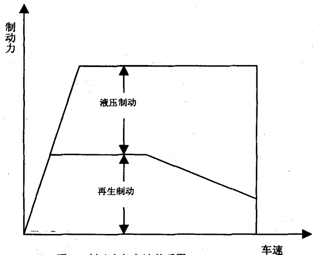
图1 制动力与车速关系图 Fig.1 Relationship between braking power and speed
