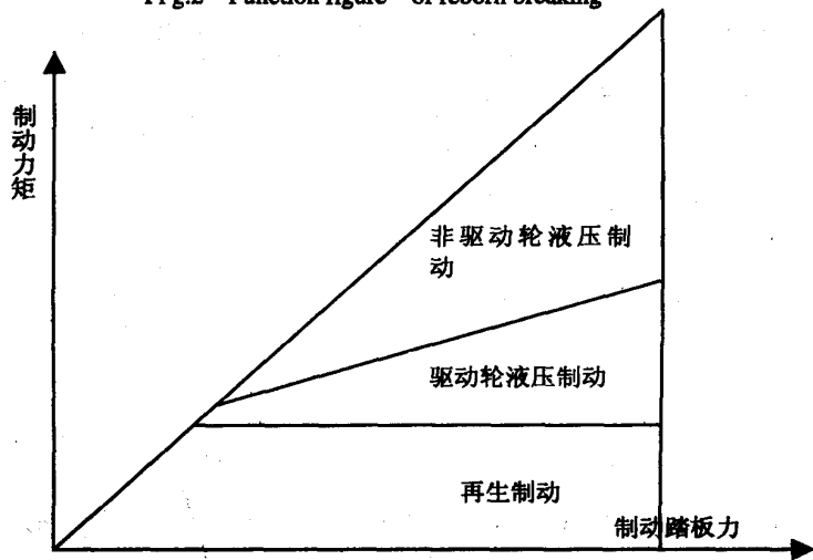
图 3 制动力矩与制动踏板力关系图 Fig.3 Relationship figure between breaking moment and pedal's power
